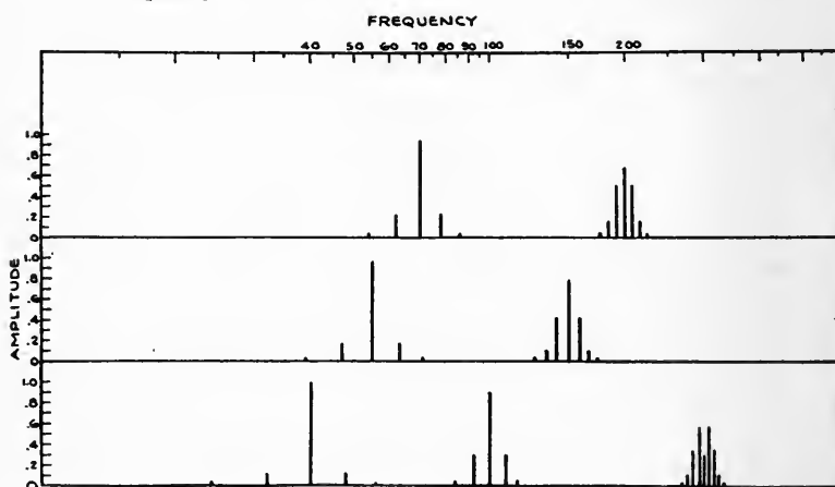
FIG. 3. Spectral distribution of warble signals: modulation \approx 5\% ; rate 8 cps; modulation sinusoidal.
